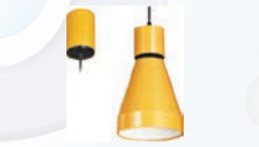
DD002 Aluminum ● COB 18W ● WH/BK/YE Mounting: Pendant Lamp Dimension: Φ 170x315
