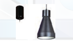
DD001 Aluminum ● COB 12W ● WH/BK/YE Mounting: Pendant Lamp Dimension: Φ 110x232
