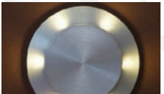
SD0202 Aluminum ● LED 1x1W ● BS Cut-out: Φ 35 Dimension: Φ 48x35
